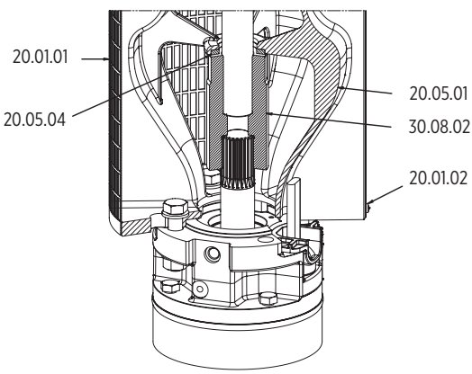
PUMP WITH 8" MOTOR
