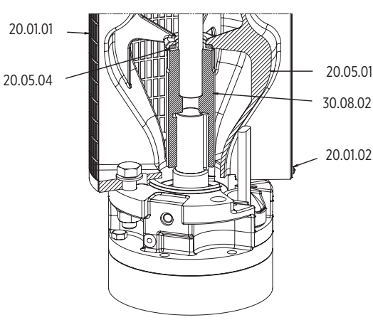
PUMP WITH 10" MOTOR
