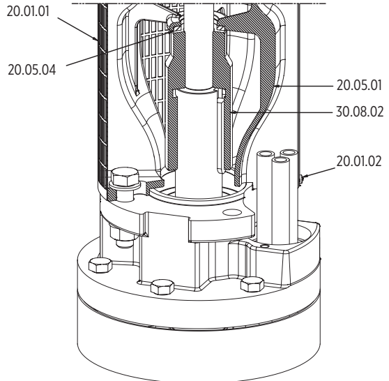
PUMP WITH 12" MOTOR
